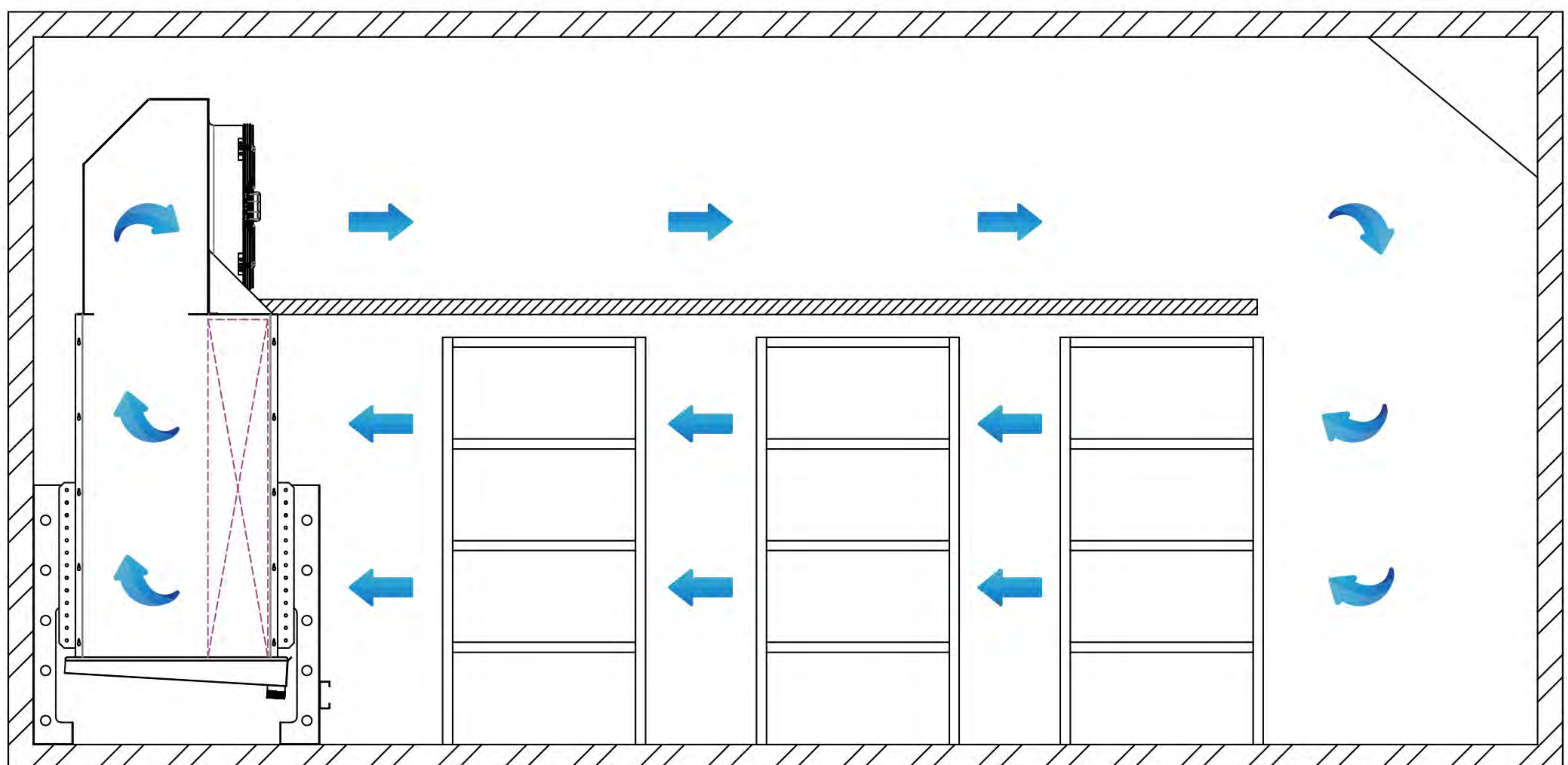
设备安装示意图及运用环境 Equipment installation diagram and operating environment
