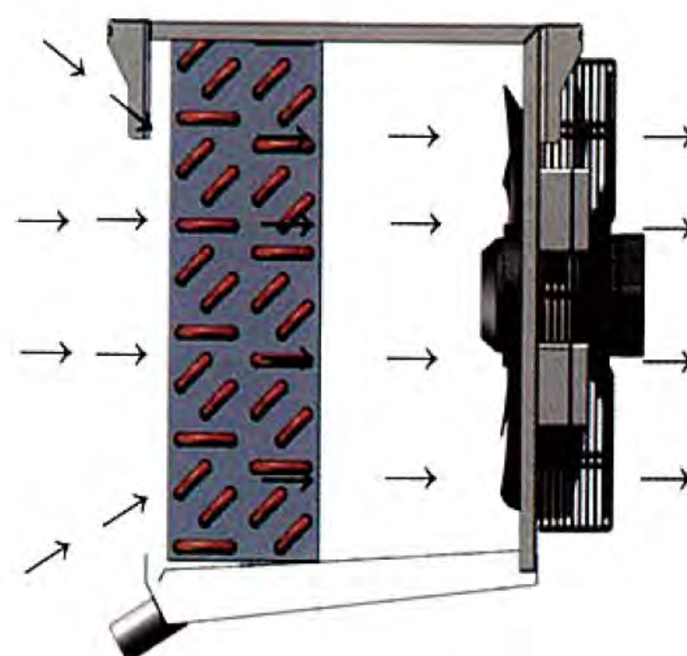
有挡风板 with windshield
